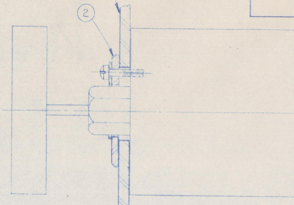
VALVE MOUNTING DETAIL TYP FOR 13 VALVES
